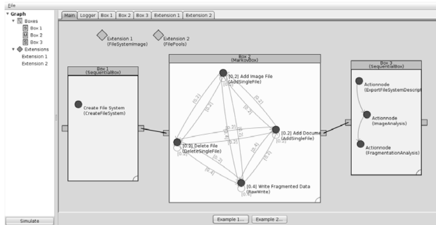
Figure 3. Screenshot of the model builder.
