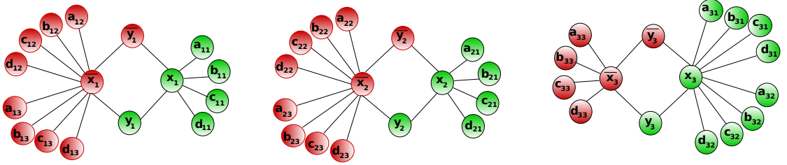
Figure 1: The three variable gadgets for the formula \Phi = (x_1 \vee x_2 \vee x_3) \wedge (x_1 \vee \bar{x}_2 \vee \bar{x}_3) \wedge (\bar{x}_1 \vee \bar{x}_2 \vee x_3) .
