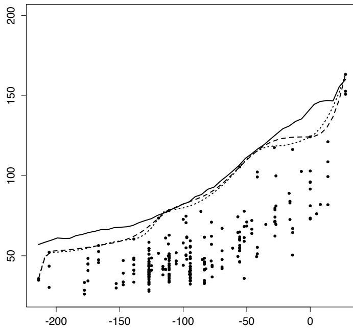
Figure 3: Scatterplot of the 254 nuclear reactor's data together with the frontier estimators: \hat{y}_{4,n}^* (solid line), CS-B (dashed line) and QS-B (dotted line).
