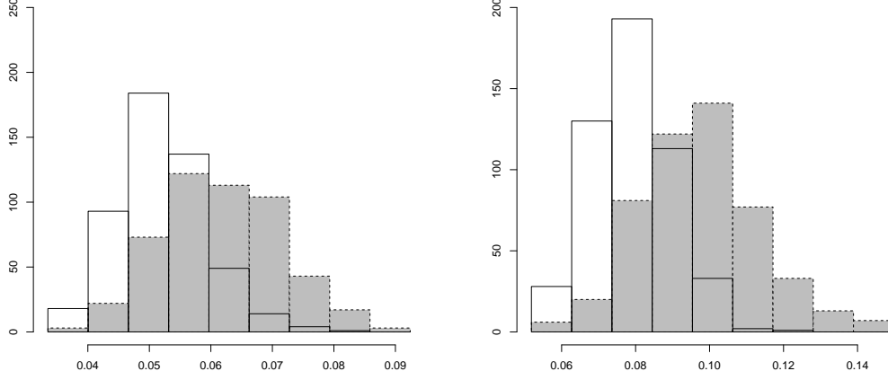
Figure 2: Comparison between the L^1 - error distributions associated with \hat{y}_{4,n}^* computed on N = 500 samples of size n = 500 . White bars: oracle strategy, grey bars: data-driven strategy, left: shape parameter \theta_1(\cdot) , right: shape parameter \theta_2(\cdot) .
