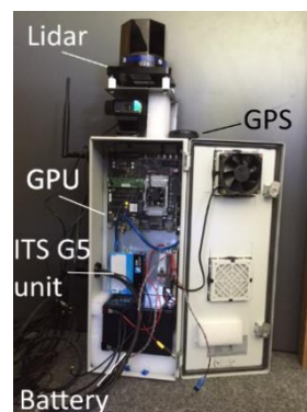
Figure 9: Perception unit hardware components.
