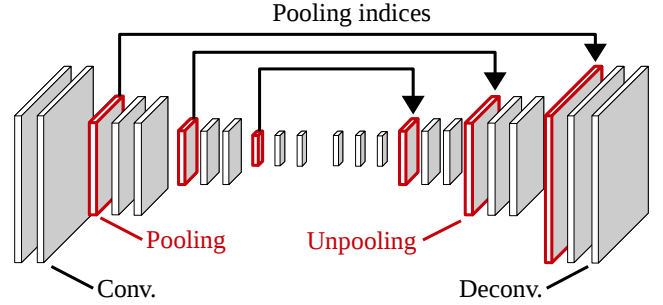
Fig. 4: Deconvolution network. The CNN is “mirrored” to learn the deconvolution.
