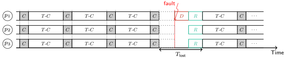
Figure 5: Behavior for a tightly coupled application.
