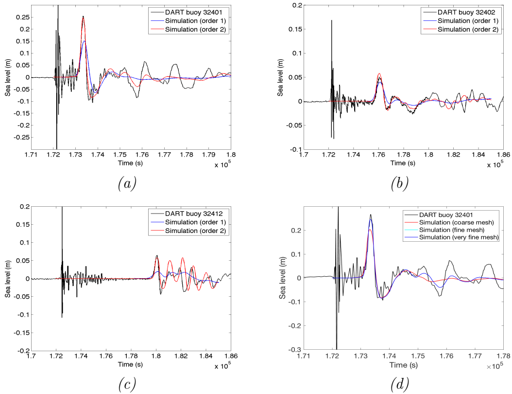
Figure 8: a), b) c) : Comparison between the sea level variations recorded by the 3 DART buoys and the corresponding simulations ( 1^{st} and 2^{nd} order schemes). d) Effect of the mesh size on the simulation accuracy for DART buoy 32401. In a), b), c), d), observations have been detided using a low pass Butterworth filter (order 4 and cutoff frequency of 4 hours), and the simulated waveforms have been filtered with the same Butterworth filter.
