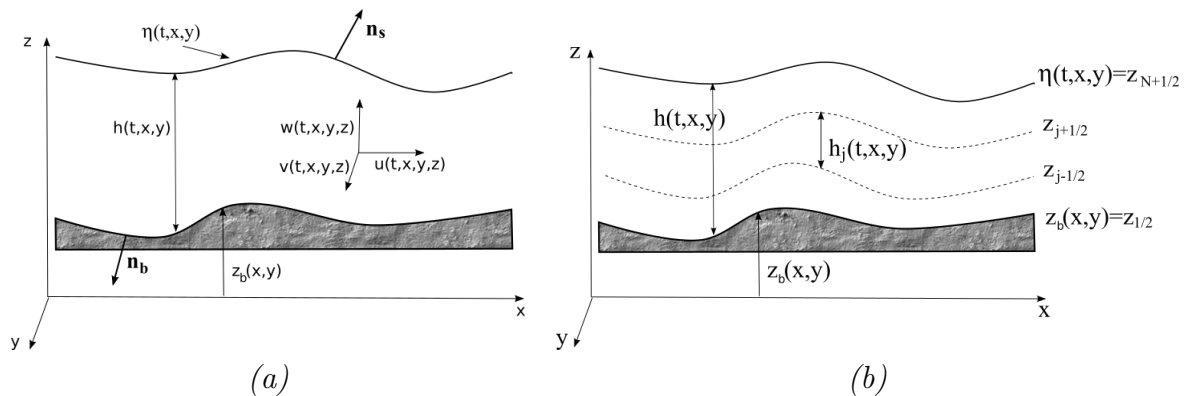
Figure 1: Fluid domain, notations and layerwise discretization.
