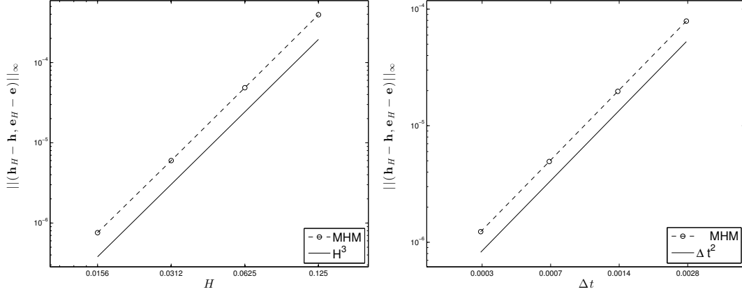
FIGURE 3. Optimal convergence history with respect to H (left) and \Delta t (right) in the \|(\mathbf{h} - \mathbf{h}_H, \mathbf{e} - \mathbf{e}_H)\|_\infty norm. Here \mathbf{\Lambda}_H = \mathbf{\Lambda}_2 .
