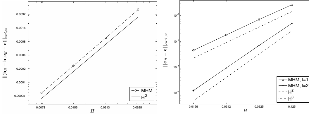
FIGURE 4. Optimal convergence history with respect to H in the \|(\mathbf{h} - \mathbf{h}_H, \mathbf{e} - \mathbf{e}_H)\|_{\text{curl},\infty} norm with \mathbf{\Lambda}_H = \mathbf{\Lambda}_2 (left). Super-convergence with respect to H for the \|\mathbf{e} - \mathbf{e}_H\|_{\text{curl},\infty} norm (right) using \mathbf{\Lambda}_H = \mathbf{\Lambda}_1 and \mathbf{\Lambda}_H = \mathbf{\Lambda}_2 .
