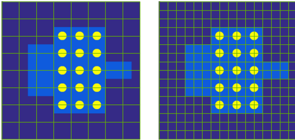
FIG. 6.8. Coarse meshes.
