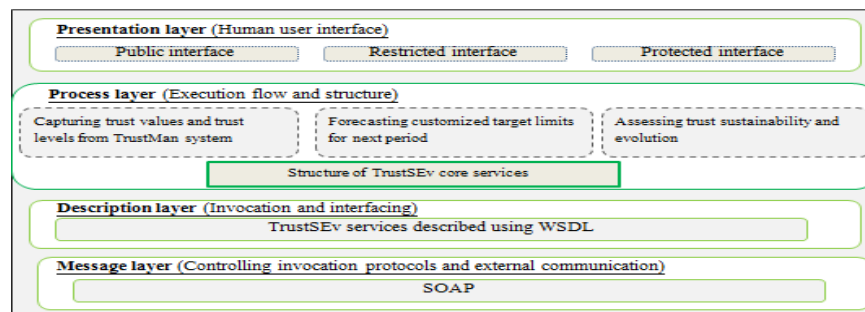
Figure 2: Four-layer Componential Architecture of the TrustSEv system
