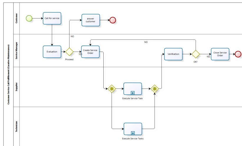
Fig. 2. Maintenance process BPMN Diagram
