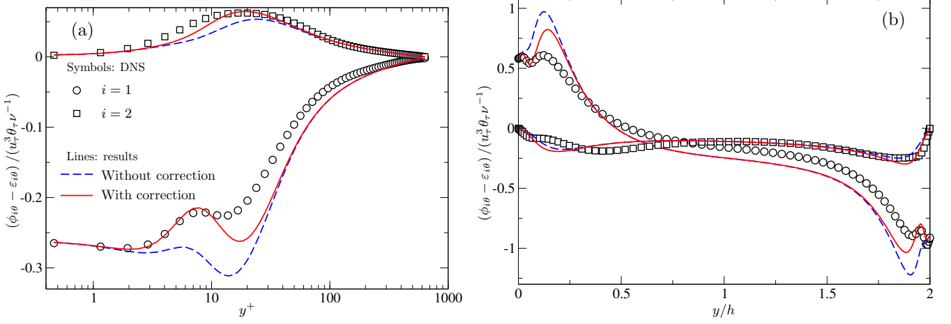
Figure 3: A priori test of the model for the difference \phi_{i\theta} - \varepsilon_{i\theta} in turbulent channel flows. (a) Forced convection regime at Re_\tau = 640 and Pr = 0.71 ; DNS of Abe et al. (2004). (b) Mixed convection regime at Re_\tau = 150 , Pr = 0.71 and Ra = 6.82 \times 10^5 ; DNS of Kasagi and Nishimura (1997) .
