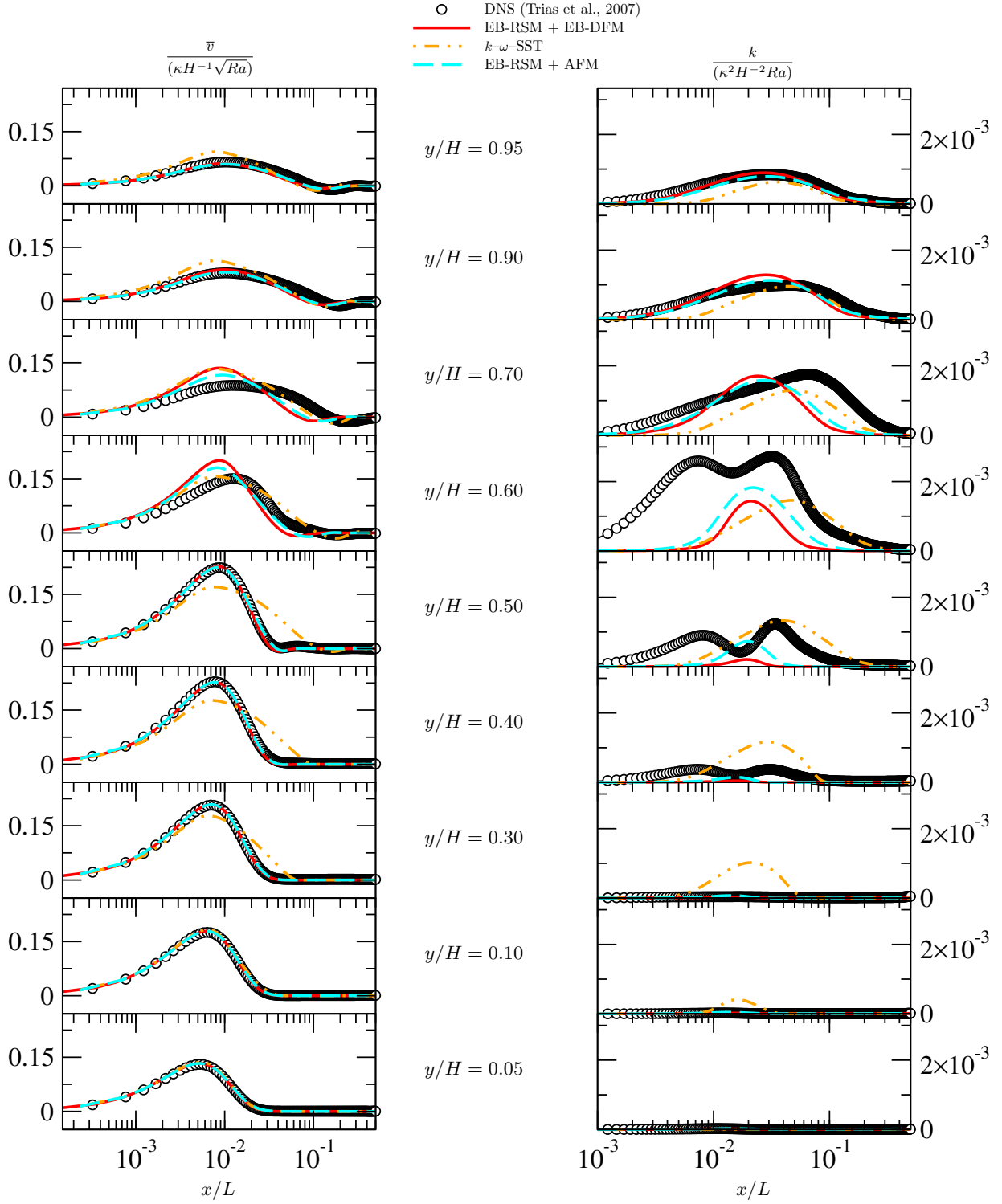
Figure 9: Differentialy heated cavity flow of Trias et al. (2007) with aspect ratio 4, Pr = 0.71 and Ra = 10^{11} . Vertical component of the mean velocity (left) and turbulent energy (right). Profiles are extracted along the wall-normal direction, on the side of the hot wall, at 9 different heights.
