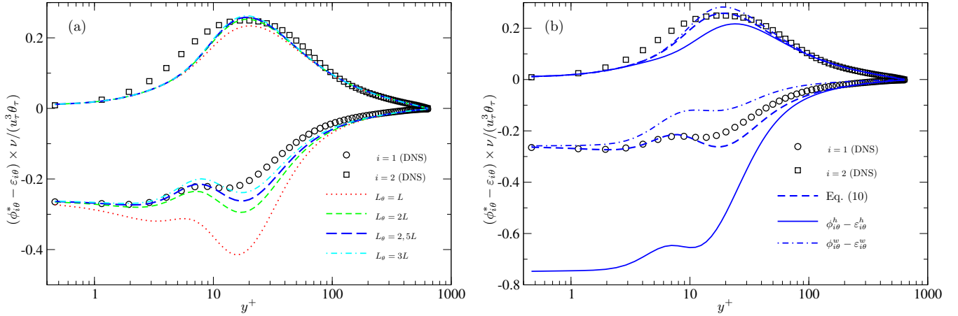
Figure 1: Channel flow in the forced convection regime of Abe et al. (2004) at Re_\tau = 640 and Pr = 0.71 . (a) A priori test of the model for \phi_{i\theta}^* - \epsilon_{i\theta} using different length scales. (b) Comparison of the quasi-homogeneous, near-wall and blended models for \phi_{i\theta}^* - \epsilon_{i\theta} in the case L_\theta = 2, 5L . A factor of 4 is applied to \phi_{2\theta}^* - \epsilon_{2\theta} for clarity.
