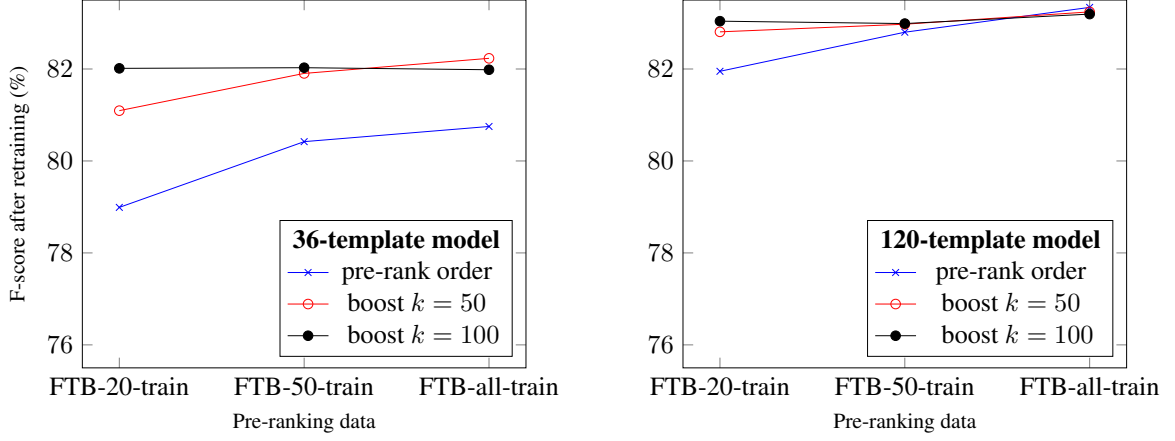
Figure 3: Average F-scores (over 5 separate runs) of selected models with a maximum size of 36 templates (left) and 120 templates (right) for different FTB pre-ranking data and different pool sizes ( k ).
