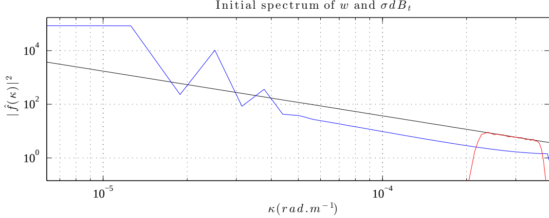
Figure 2: Spectrum ( m^2.s^{-2}/(rad.m^{-1}) ) of w , at the initial time, in blue, spectrum of \sigma_H \dot{B} (up to a multiplicative constant), in red, and slope -\frac{5}{3} in black. In the simulation performed, \sigma_H \dot{B} is restricted to a narrow spectral band. Thus, this velocity component almost only acts near the resolution cutoff, where the large-scale component, w , has a low energy.
