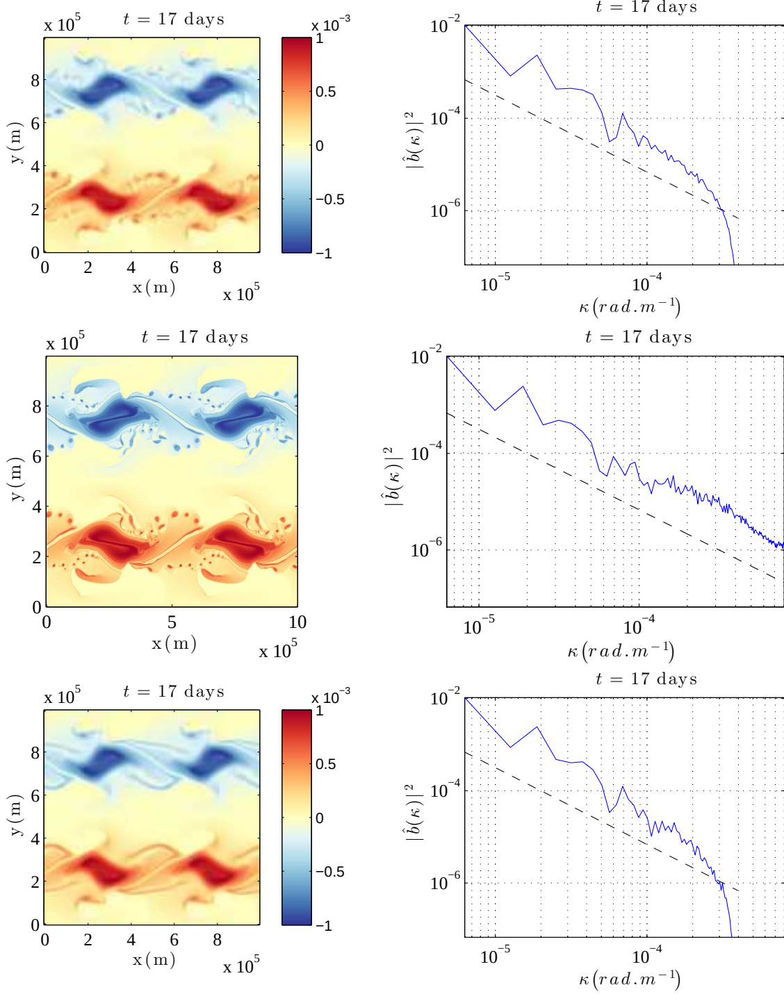
Figure 3: Buoyancy ( m.s^{-2} ) and its spectrum ( m^3.s^{-4}/(rad.m^{-1}) ) at the 17 th day of advection for SQG MU at resolution 128^2 (top), SQG at resolution 512^2 (middle) and at resolution 128^2 (bottom). Unlike SQG MU , the low-resolved SQG simulation diffuses the “pearl necklaces”, noticeable only at higher resolution.
