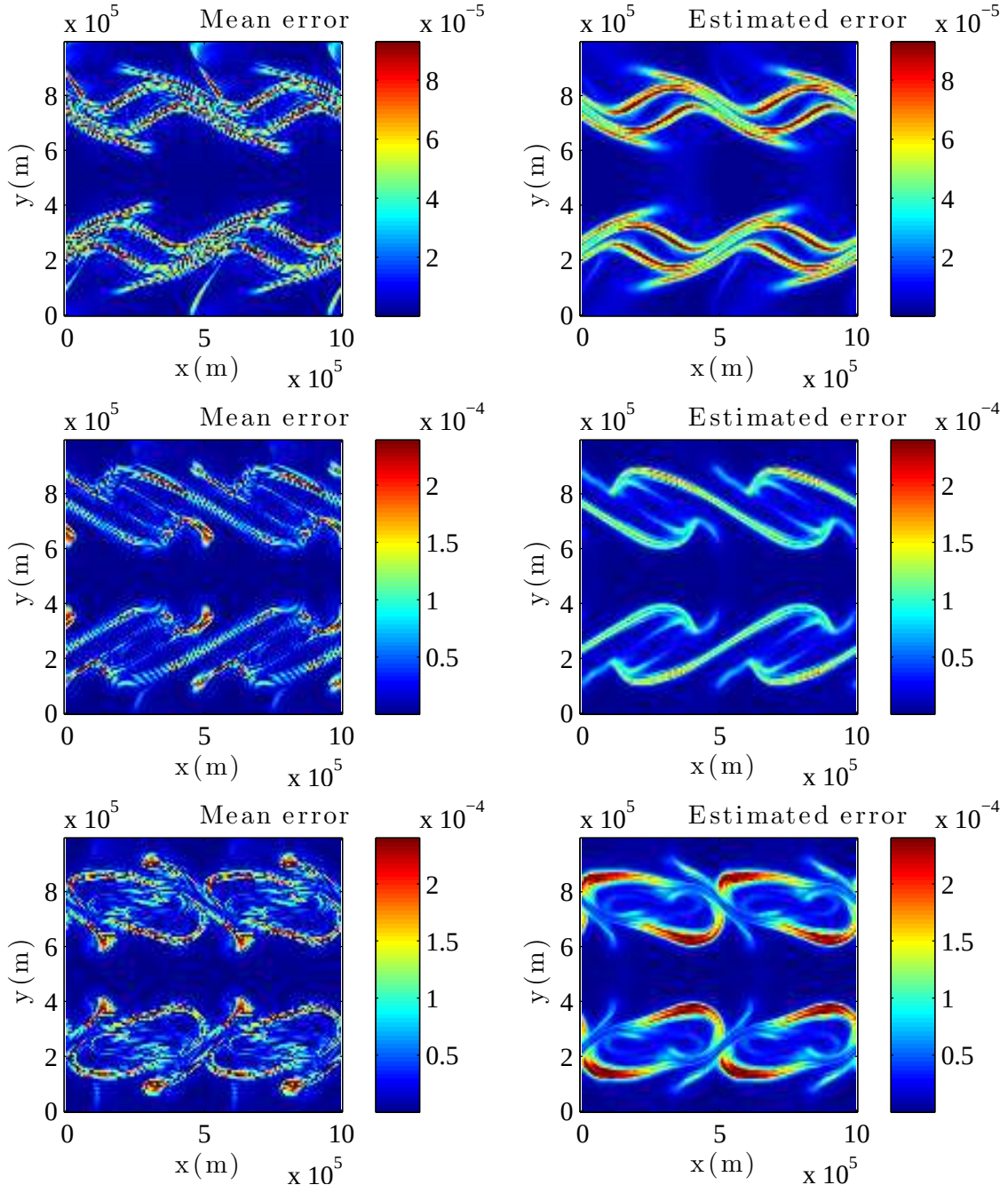
Figure 5: Buoyancy bias absolute value, e = |\hat{\mathbb{E}}\{b\} - b^{ref}| , ( m.s^{-2} ) of the SQG MU model (left) and its estimation, \epsilon_{est} , ( 1.96 \times the standard deviation of the ensemble) (right) at resolution 128^2 at (from top to bottom) t = 10, 13 and 15 days of advection. The reference is the usual SQG model at resolution 512^2 – adequately filtered and subsampled.
