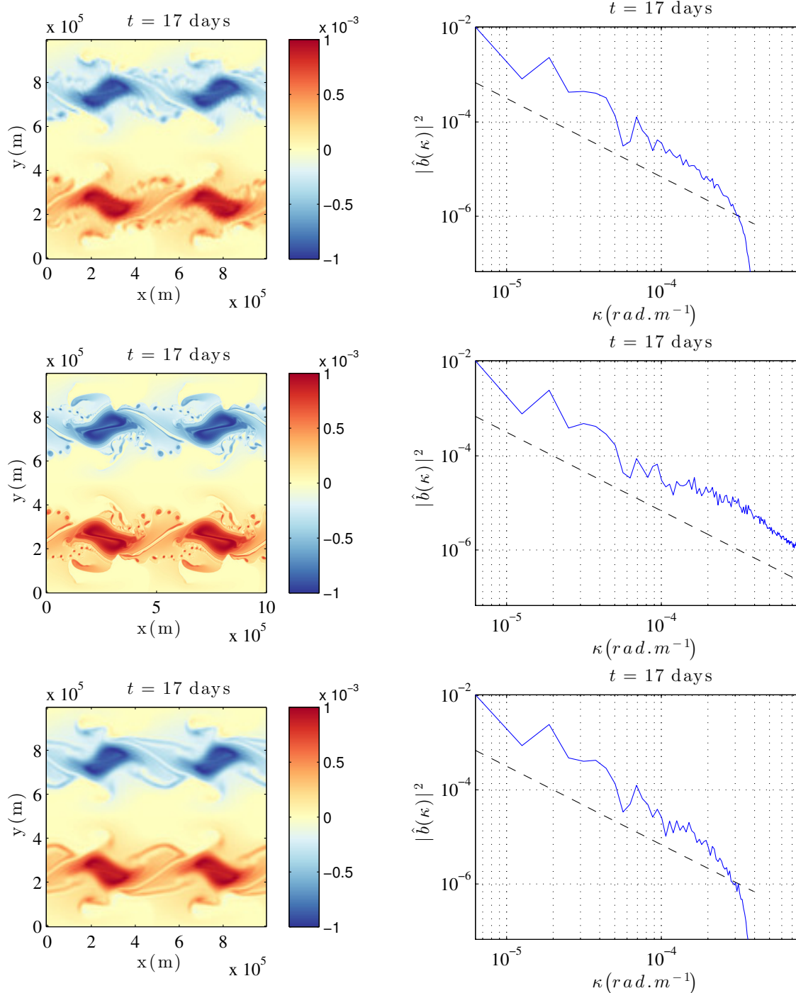
Figure 3: Buoyancy ( \text{m.s}^{-2} ) and its spectrum ( \text{m}^2.\text{s}^{-4}/(\text{rad.m}^{-1}) ) at the 17 th day of advection for SQGMU at resolution 128^2 (top), SQG at resolution 512^2 (middle) and at resolution 128^2 (bottom). Unlike SQGMU, the low-resolved SQG simulation diffuses the “pearl necklaces”, noticeable only at higher resolution (Colour online).
