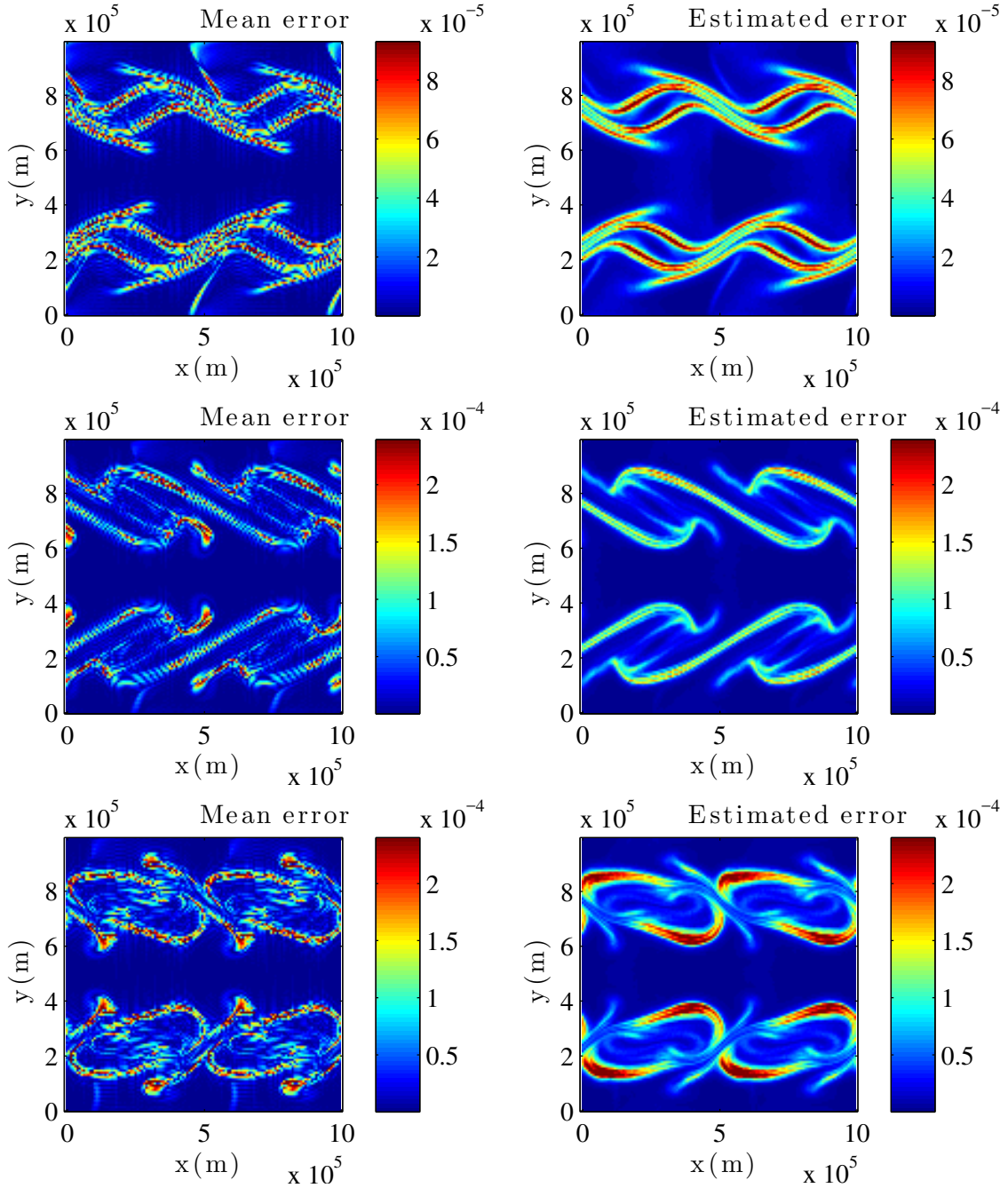
Figure 5: Buoyancy bias absolute value, e = |\widehat{\mathbb{E}}\{b\} - b^{ref}| , ( \text{m}\cdot\text{s}^{-2} ) of the \text{SQG}_{\text{MU}} model (left) and its estimation, \epsilon_{est} , ( 1.96 \times the standard deviation of the ensemble) (right) at resolution 128^2 at (from top to bottom) t = 10, 13 and 15 days of advection. The reference is the usual SQG model at resolution 512^2 – adequately filtered and subsampled (Colour online).
