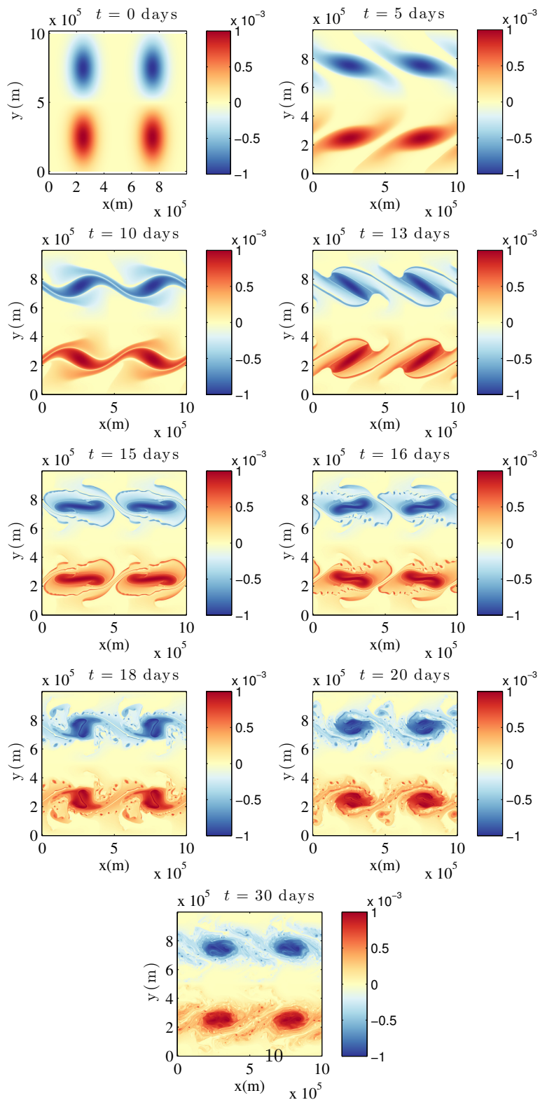
Figure 1: Buoyancy ( m \cdot s^{-2} ) at t = 0, 5, 10, 13, 15, 16, 20, 30 days of advection for the usual SQG model at resolution 512^2 (Colour online).
