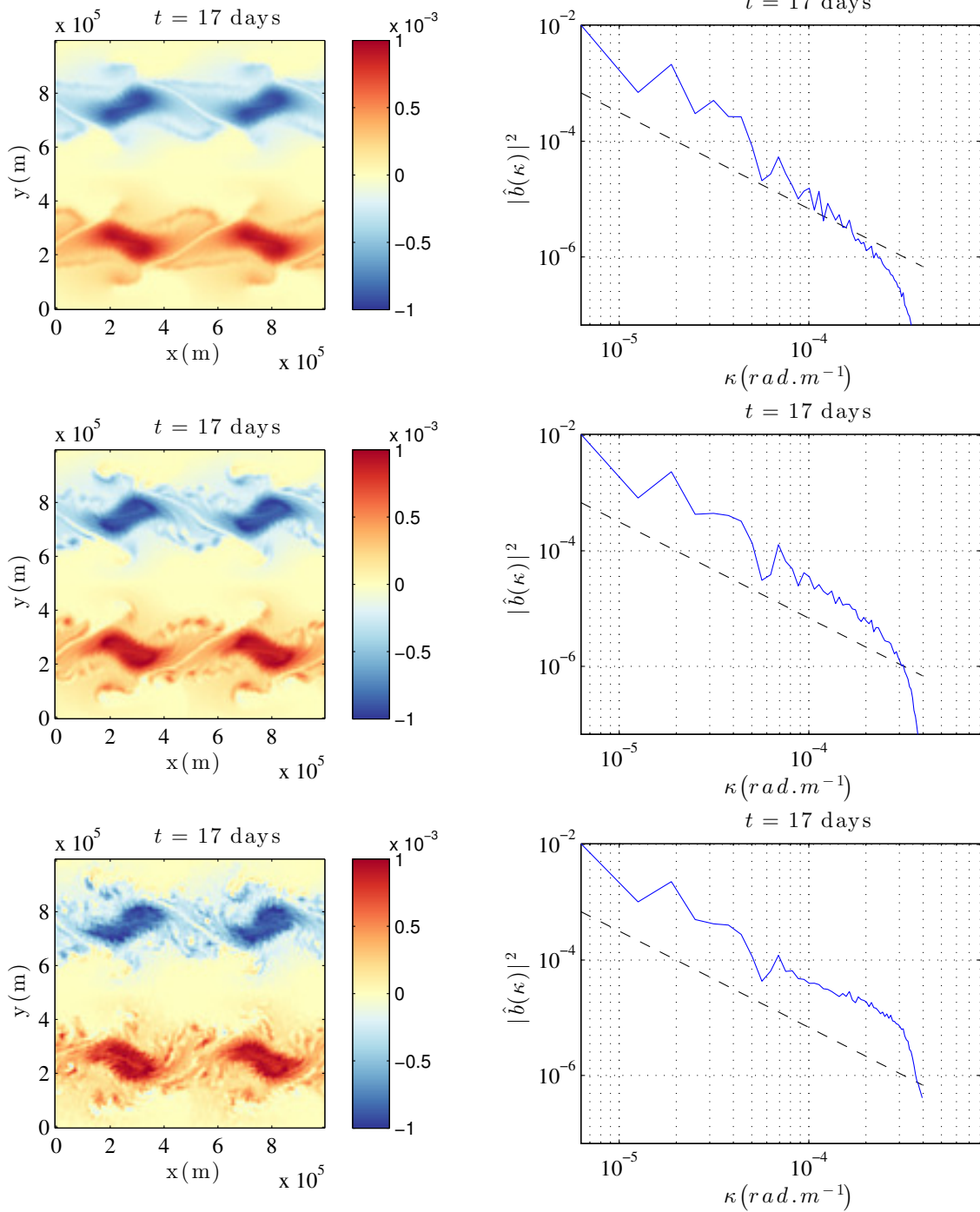
Figure 4: Buoyancy ( \text{m.s}^{-2} ) and its spectrum ( \text{m}^2.\text{s}^{-4}/(\text{rad.m}^{-1}) ) at the t = 17^{\text{th}} day of advection for the SQG MU model with a small-scale velocity component three times weaker than the one prescribed by the diffusion coefficient a_H (top), with the correct amount of small-scale energy (middle) and a small-scale velocity three times higher than the model diffusion. If the prescribed balance between noise and diffusion is not met the tracer field becomes quickly too smooth or too noisy (Colour online).
