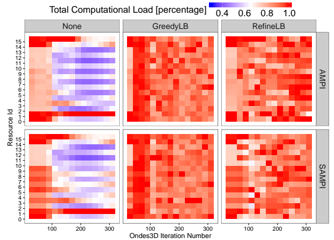
(b) Per-process computational load of the Ligurian workload.
