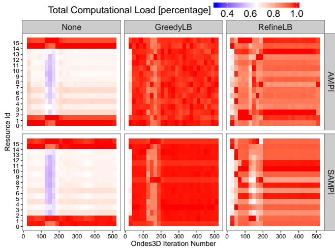
(a) Per-process computational load of the Chuetsu-Oki workload.
