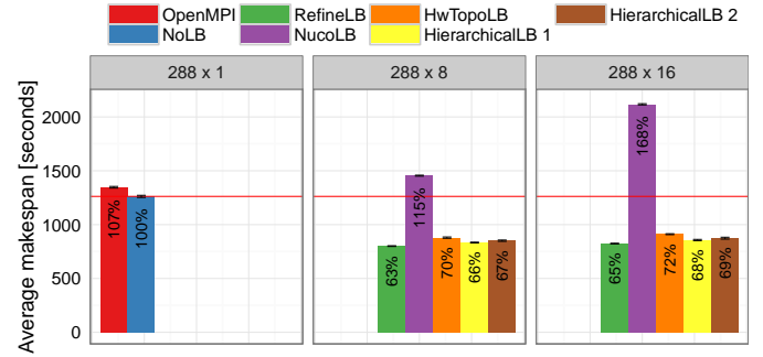
Figure 4: Mean execution time of Ondes3D on 288 cores with different task granularities (VP counts) and load balancers.
