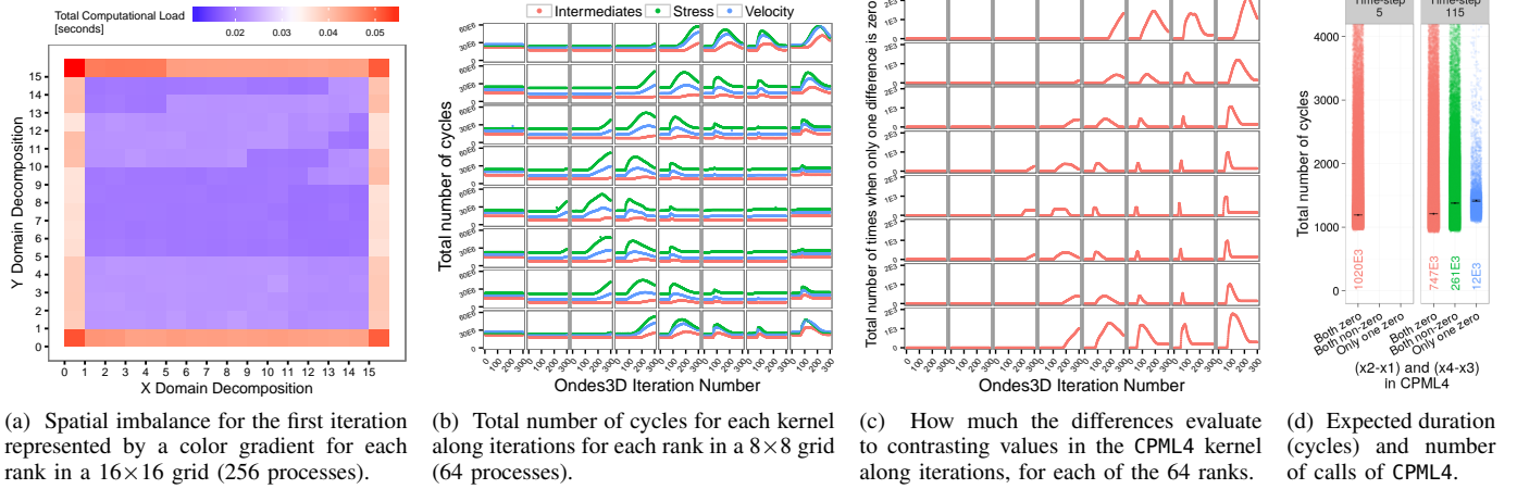
Figure 2: Load imbalances for the Ligurian workload: (a) spatial load imbalance; (b) temporal load imbalance for three kernels; (c) CPML4 substrate values evaluating to distinct values; and (d) explaining temporal anomaly with CPML4 argument analysis.
