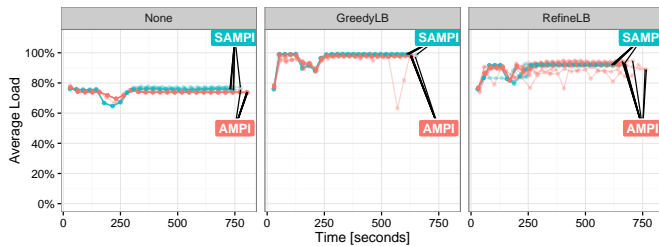
(c) Average Load and makespan using the Chuetsu-Oki workload.
