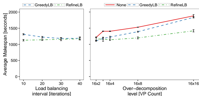
Figure 7: Simulated makespan predictions for the Ligurian earthquake simulation with (left) four load balancing intervals (in number of iterations) and (right) with five over-decomposition levels (2, 3, 4, 8, and 16) on 16 cores.
