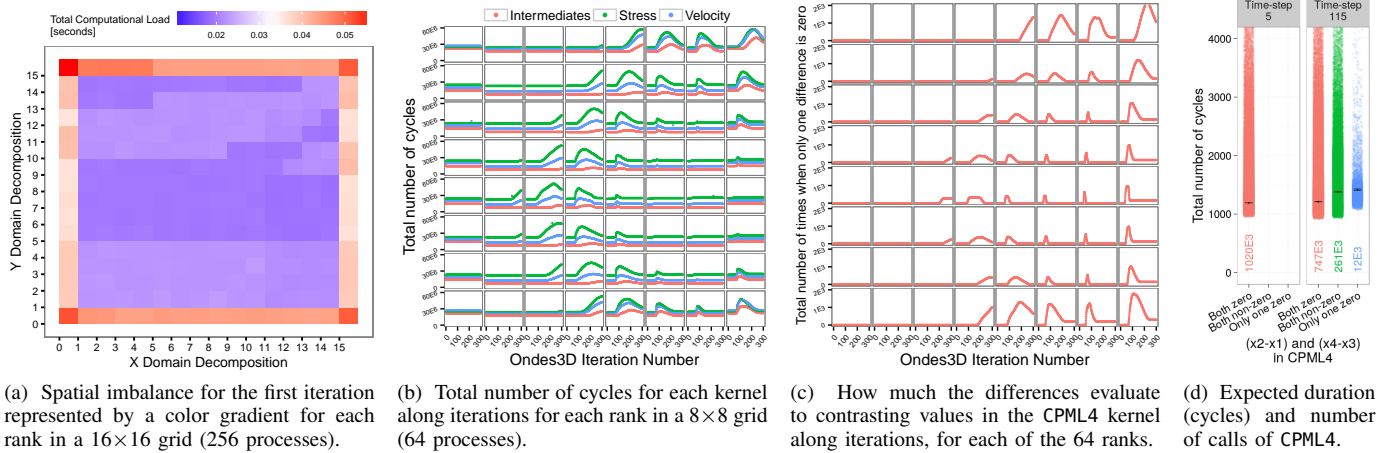
Figure 2: Load imbalances for the Ligurian workload: (a) spatial load imbalance; (b) temporal load imbalance for three kernels; (c) CPML4 substrate values evaluating to distinct values; and (d) explaining temporal anomaly with CPML4 argument analysis.
