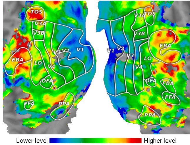
B Fingerprint summaries for Huth2012
