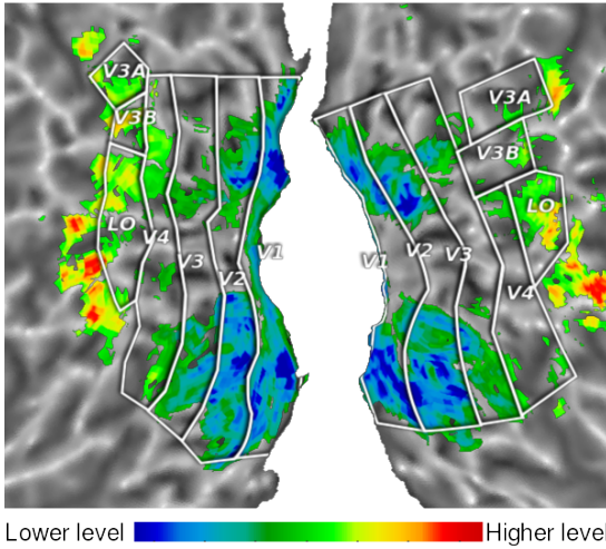
A Fingerprint summaries for Kay2008
