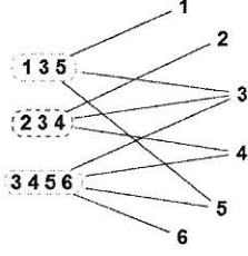
Figure 2: Clique cover graph for the ECC in Fig. 1(ii).
