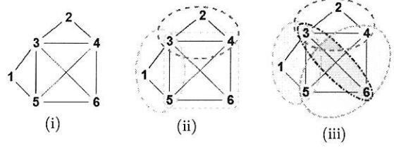
Figure 1: Graph (i) taken from [15], and two examples of ECCs in (ii) and (iii).
