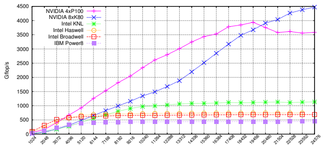
Fig. 6. Task-based QDWH performance across various architectures.
