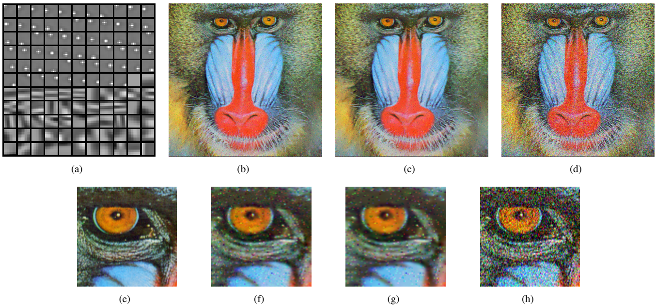
Fig. 6. Sparsity-Constrained DOLPHIn example: Image original is the 512 \times 512 RGB “mandrill” picture, measurements are noisy CDPs (obtained using two complex-valued octanary masks, noise-SNR 10 dB, per color channel), \mu_1 = 0.003 m_Y , \mu_2 = 0.00504 m_Y (other parameters as described in Section IV-G). \mathbf{D}_{(0)} = (\mathbf{I}, \mathbf{F}_D) for R-channel, final dictionary then served as initial dictionary for G-channel, whose final dictionary in turn was initial dictionary for B-channel; \mathbf{X}_{(0)} \in \mathcal{X} random for each channel. (a) final dictionary (excerpt) for B-channel (b) image reconstruction \mathbf{X}_{\text{DOLPHIn}} , (c) image reconstruction \mathcal{R}(\mathbf{DA}) from sparsely coded patches, (d) reconstruction \mathbf{X}_{\text{WF}} after 50 WF iterations. Final PSNR values: 20.53 dB for \mathcal{R}(\mathbf{DA}) , 20.79 dB for \mathbf{X}_{\text{DOLPHIn}} , 14.47 dB for \mathbf{X}_{\text{WF}} ; final SSIM values: 0.4780 for \mathcal{R}(\mathbf{DA}) , 0.5242 for \mathbf{X}_{\text{DOLPHIn}} , 0.2961 for \mathbf{X}_{\text{WF}} ; average \|\mathbf{a}^i\|_0 is 5.30. (Means over all color channels.) (e)–(h): zoomed-in 100 \times 100 pixel parts (magnified) of (e) original image, (f) \mathbf{X}_{\text{DOLPHIn}} , (g) \mathcal{R}(\mathbf{DA}) and (h) \mathbf{X}_{\text{WF}} .
