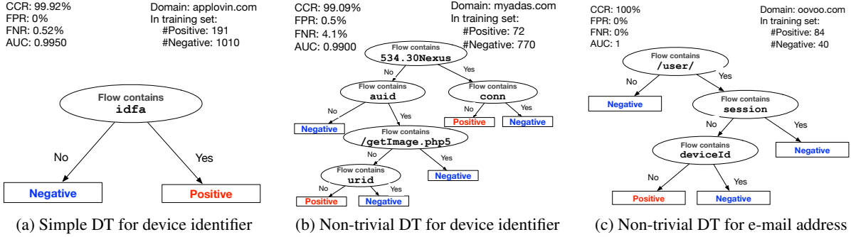
Figure 4: Example decision trees (DTs) for ReCon’s per-domain per-OS classifiers. The classifier begins at the root (top) node, and traverses the tree based on whether the term at each node is present. The leaves (boxes) indicate whether there is a PII leak (positive) or not (negative) for each path. The top right of each figure shows the number of positive/negative samples used to train each DT.
