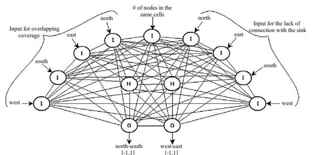
Fig. 3. Neural network architecture of one node
