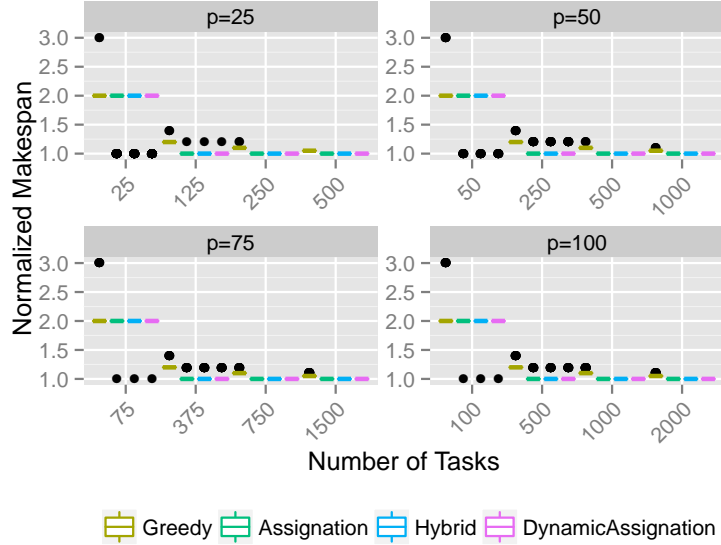
Figure 5: Normalized Makespan for tasks of type Homogeneous.
