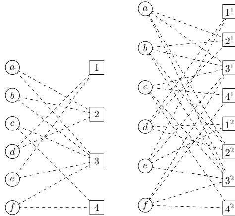
Figure 2: An example of replication of a bipartite graph. On the left G , on the right G^2 .
