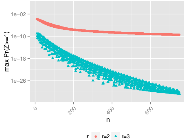
Figure 4: \max_{p \in [1, n]} Pr(Z \geq 1) in function of n (with logarithm scale on y-axis).
