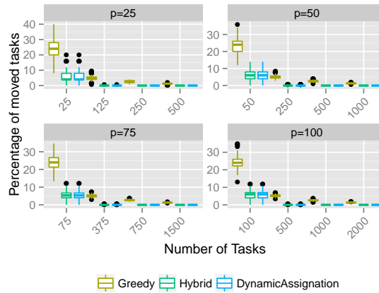
Figure 7: Percentage of non local tasks for tasks of type Homogeneous.
