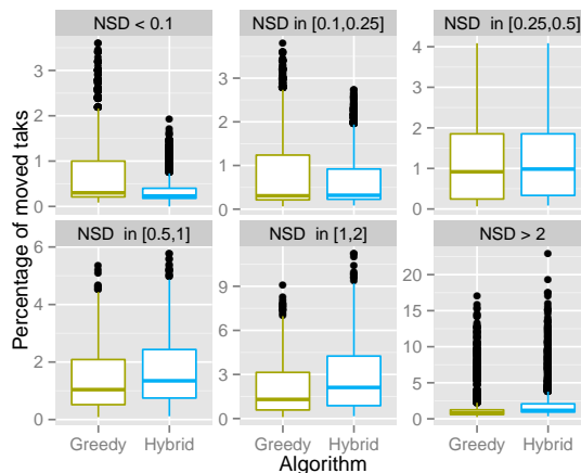
Figure 10: Percentage of moved tasks for jobs with more than 500 tasks according to several value of normalized standard deviation (NSD)
