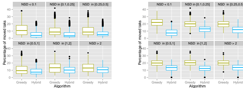
(a) Percentage of non local tasks for jobs with less than 500 tasks
