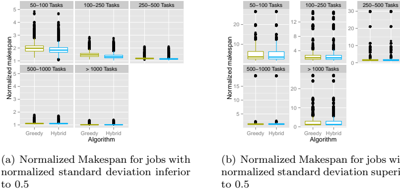
Fig. 11: Normalized Makespan according to several categories of number of tasks
