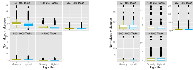
(a) Normalized Makespan for jobs with normalized standard deviation inferior to 0.5
