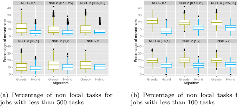
Fig. 9: Percentage of non local tasks according to several values of normalized standard deviation (NSD)
