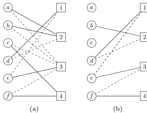
Fig. 3: Example of Alternating path.
