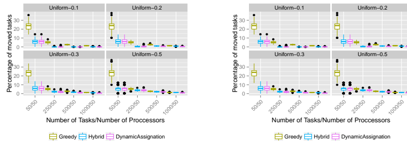
(a) Percentage of moved tasks for tasks of type Uniform.
