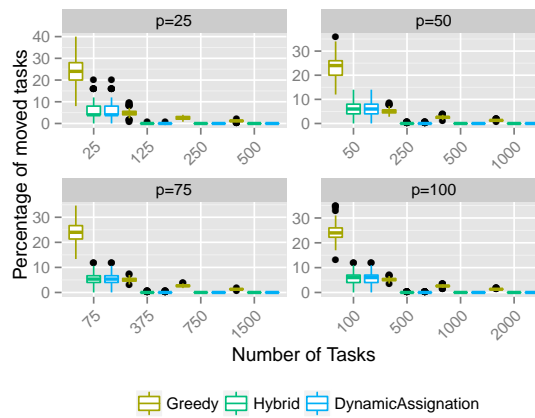
Fig. 7: Percentage of non local tasks for tasks of type Homogeneous.
