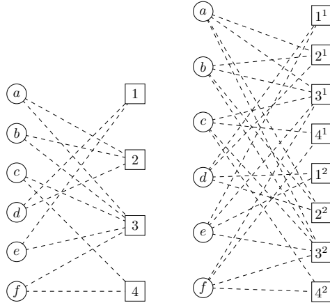
Fig. 2: An example of replication of a bipartite graph. On the left G , on the right G^2 .
