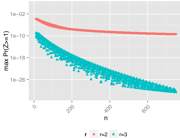
Fig. 4: \max_{p \in [1, n]} Pr(Z \geq 1) in function of n (with logarithm scale on y-axis).
