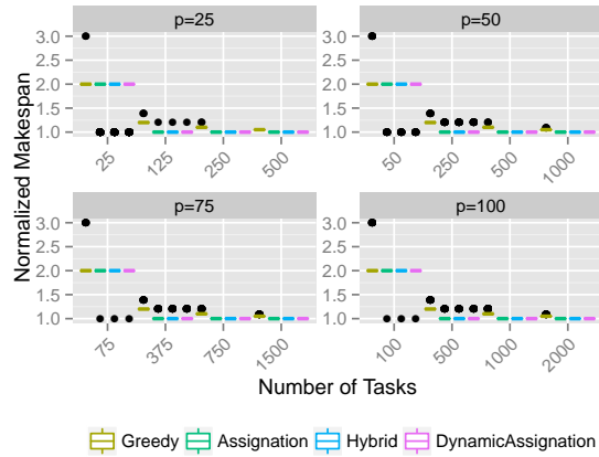
Fig. 5: Normalized Makespan for tasks of type Homogeneous.
