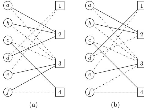
Fig. 1: Two examples of assignments for the same problem.
