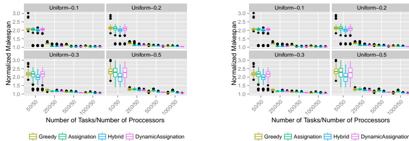
(a) Normalized Makespan for tasks of type Uniform.
