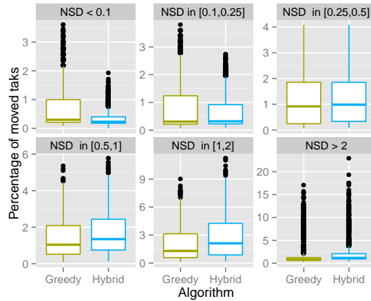
Fig. 10: Percentage of moved tasks for jobs with more than 500 tasks according to several value of normalized standard deviation (NSD)
