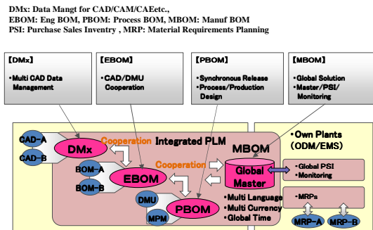
Fig.3 Architecture of integrated PLM system
