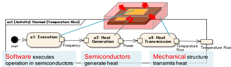
Fig. 3 Temperature rise in an electronic product
