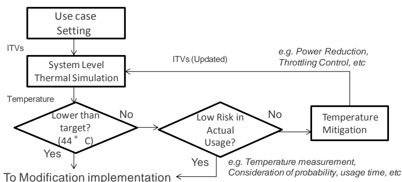
Fig. 8 Verification workflow
