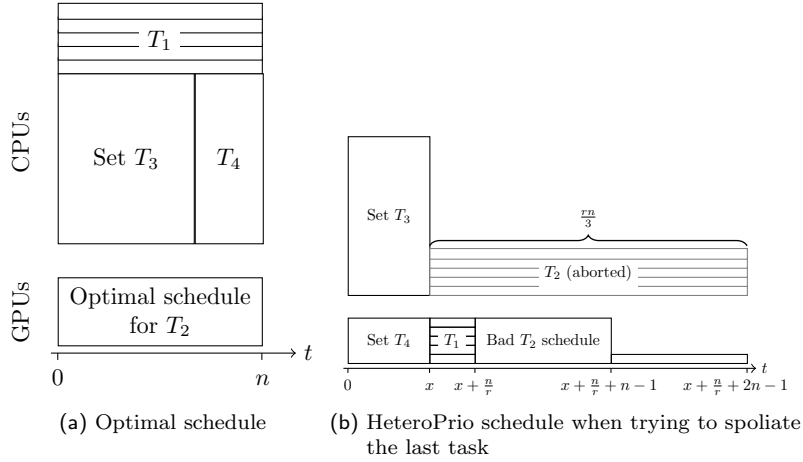
Fig. 5: Optimal and HeteroPrio schedules for the instance of Theorem 14.
