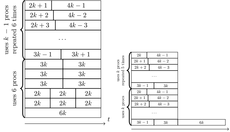
Fig. 4: Two schedules for task set T_2 on n = 6k homogeneous processors. Tasks are labeled with their processing times.
