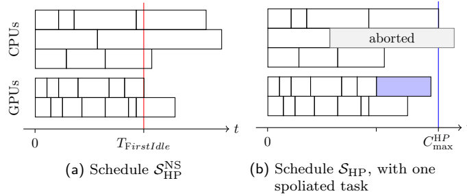
Fig. 1: Example of a HeteroPrio schedule
