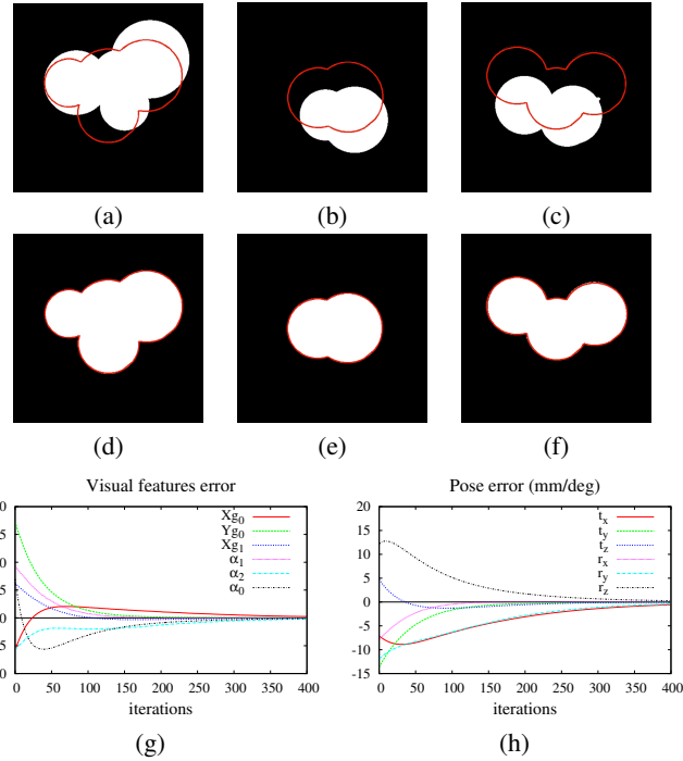
Fig. 3. Positioning task using six geometric features measured in three orthogonal images. (a-c) Initial object cross-section with the desired contour to reach (in red). (d-f) Observed object cross-sections at convergence of the algorithm. (g,h) Minimization of the visual and pose errors.
