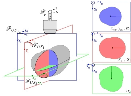
Fig. 2. The visual features are computed from three orthogonal planes. The probe frame coincides with the frame of US_0 . On the right, this frame is reprojected in the various image plane frames. (Note that in this illustration the origins of the frames \mathcal{F}_p and \mathcal{F}_{US_i} are shifted for better visibility whereas they are superimposed in practice.)
