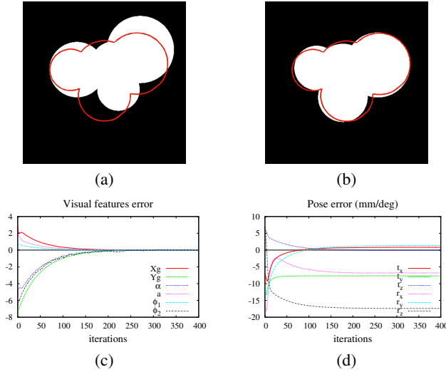
Fig. 1. Positioning task with mono-plane approach. (a,b) Initial and final cross-sections of the object (in white) with the desired contour superimposed (in red). The convergence in terms of visual error (c) does not correspond to the convergence in pose of the algorithm.
