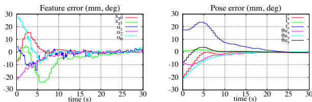
Fig. 7. Positioning task with six features extracted from three orthogonal images. Decrease of the visual error (left) and pose error (right) during the visual servoing.
