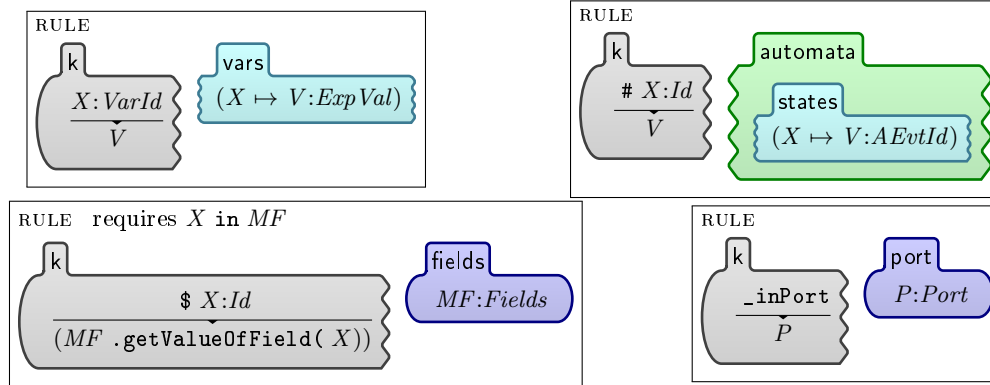
Figure 10: GPFL's semantics for variables
