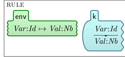
Figure 3: Peano's \mathbb{K} rule for variables
