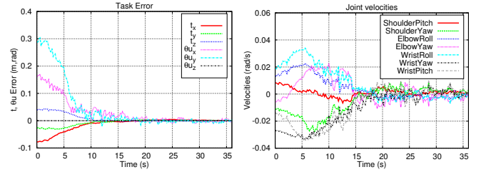
Fig. 8. Task error and joint velocities of Romeo's left arm while grasping a can using PBVS and adding some bias. The bias added to the estimated extrinsic parameters were: 3cm in each translation axis and 2 degrees in rotation. The bias added to the camera intrinsic parameters were: +40 pixels in the focal lengths and +10 pixels in the principal point.
