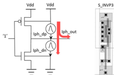
Fig. 15. (left) Laser-induced effect in an inverter, and (right) Inverter-based detector cell S_INVVP3
