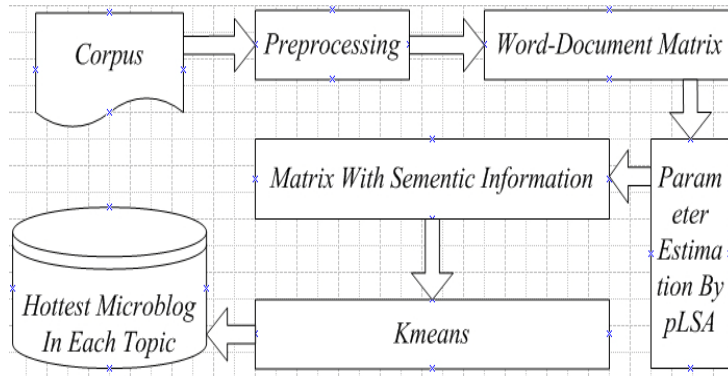
Figure 1. Algorithm process
