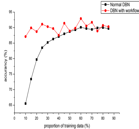
Fig. 7. Identification Accuracy
