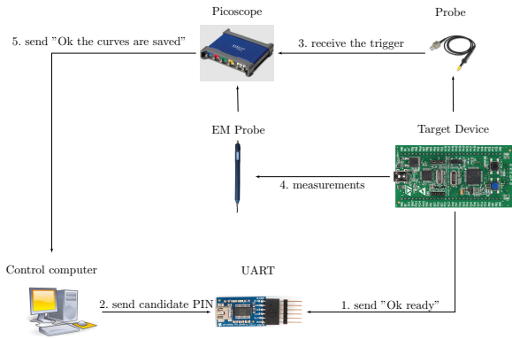
Figure 1: Experimental bench
