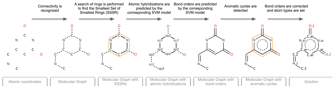
Figure 1: Schematic workflow of the Knodle algorithm.
