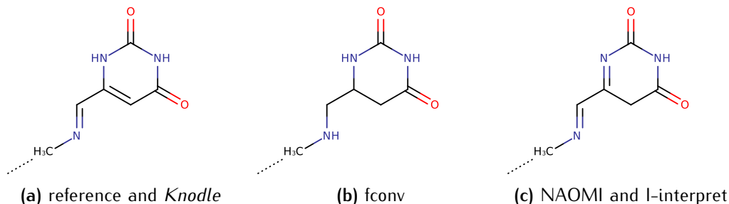
Figure 6: Perception of the 3fcf structure, an example of an aromatic heterocycle with two exocyclic sp 2 -hybridized oxygens. NAOMI, I-interpret, and fconv incorrectly predict hybridization of one of the cycle's carbons.
