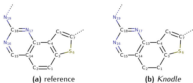
Figure 5: Perception of the 3qgy structure. Here, Knodle does not recognize aromaticity of the nonplanar C1-C2-C14-C13-C4-C3 ring, where the value of the C3-C1-C2-C14 dihedral angle is of about 23°.
