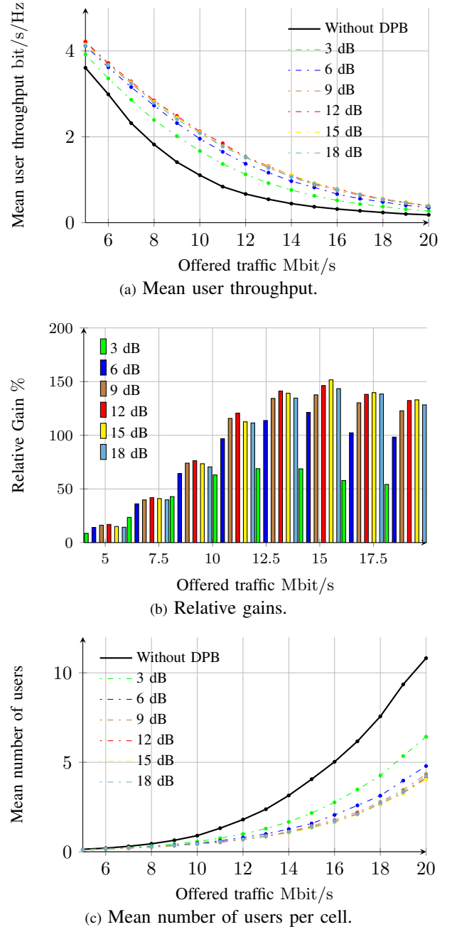
Fig. 5. Throughput performance obtained by system-level simulation for dynamic clustering DPB.
