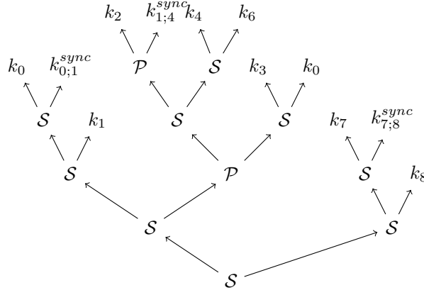
Figure 7: Serie-Parallel tree decomposition of the example of program of Figure 4
