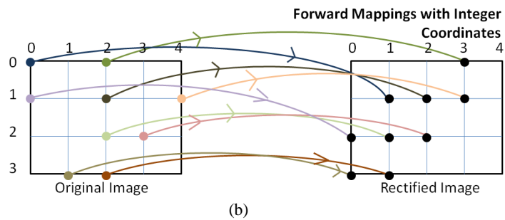
Fig. 4. Third step of the compression flow (a) selection of nearest source pixels from fractional inverse mapping (b) extraction of forward mapping with integer coordinates
