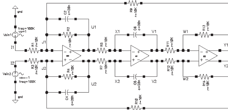
Fig. 2. Biquadratic Filter
