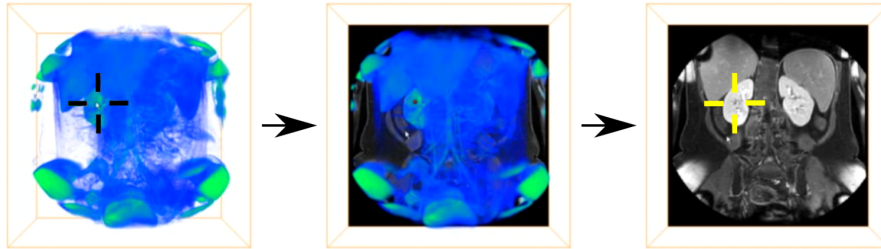
Fig. 10 What you see is what you pick interaction [86]. Once a location is picked in the projected view of a volumetric visualization (left), its 3D location is deduced and a cutting plane can be placed accordingly, facilitating the exploration of this cutting plane in the context of the volume rendering (center) or by itself (right). Image courtesy of and © Alexander Wiebel, used by permission.
