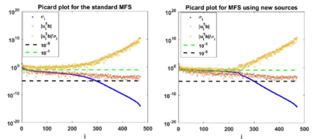
Fig. 2: DPC plot example for the scar patient (case c-d of fig. 1), for an instant of time t_k of interest. Left: for the standard MFS problem. Right: for the MFS problem using new sources.
