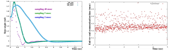
Figure 7: a) Knee position – b) End-to-end delay
