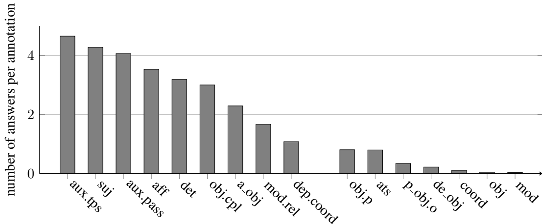
Figure 4: Density of answers for each relation on the REF_{Eval} corpus (a whitespace separates relations where density is greater than 1 from the others).
