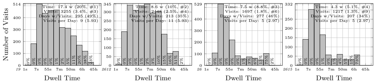
Figure 5: Visit dwell time histogram for e7d 's top towers. The number at the bottom of each bar is the portion of time that the visits constitute. Inset in each figure are the total time and total visits to the tower as well as the number of days with visits and the median visits per day for days on which the tower was visited at least once and the corresponding MAD.
