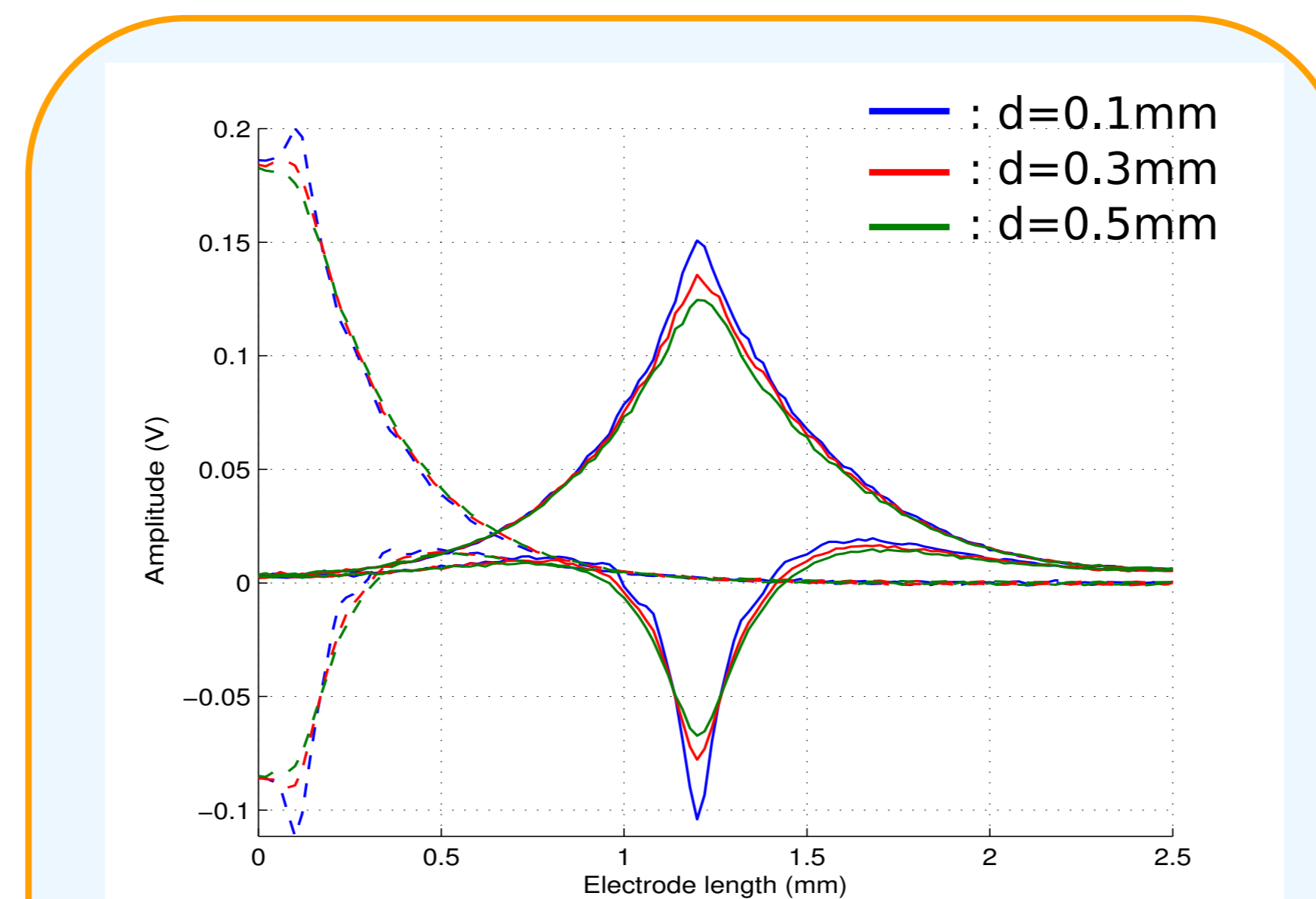
Figure 5. Voltage distribution along the electrode array. d is the radial distance from the electrode.
