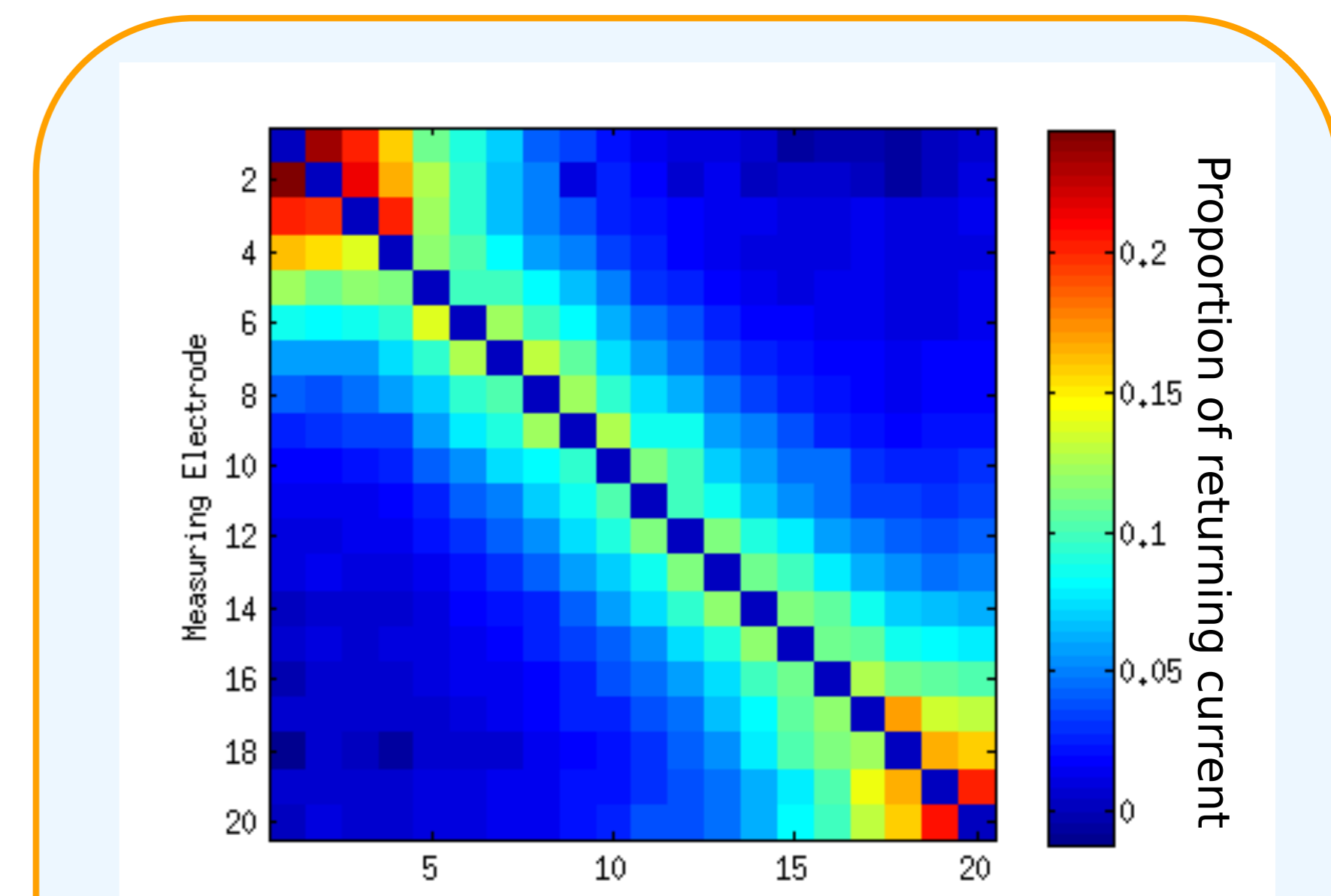
Figure 6. Returning current distribution from in situ measurements
