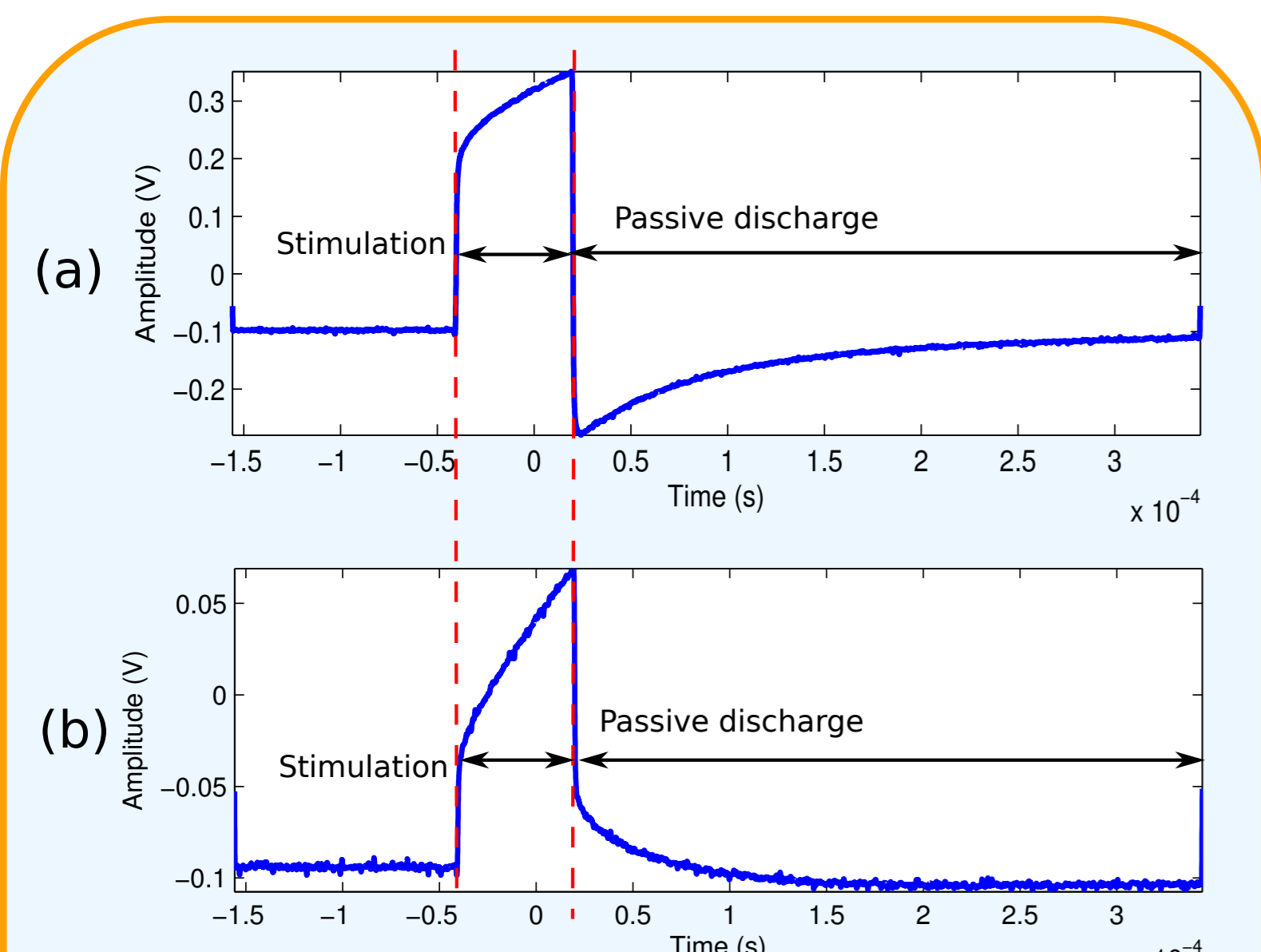
Figure 4. Stimulation waveform measured from: (a) near a stimulating electrode; (b) near a non-stimulating electrode
