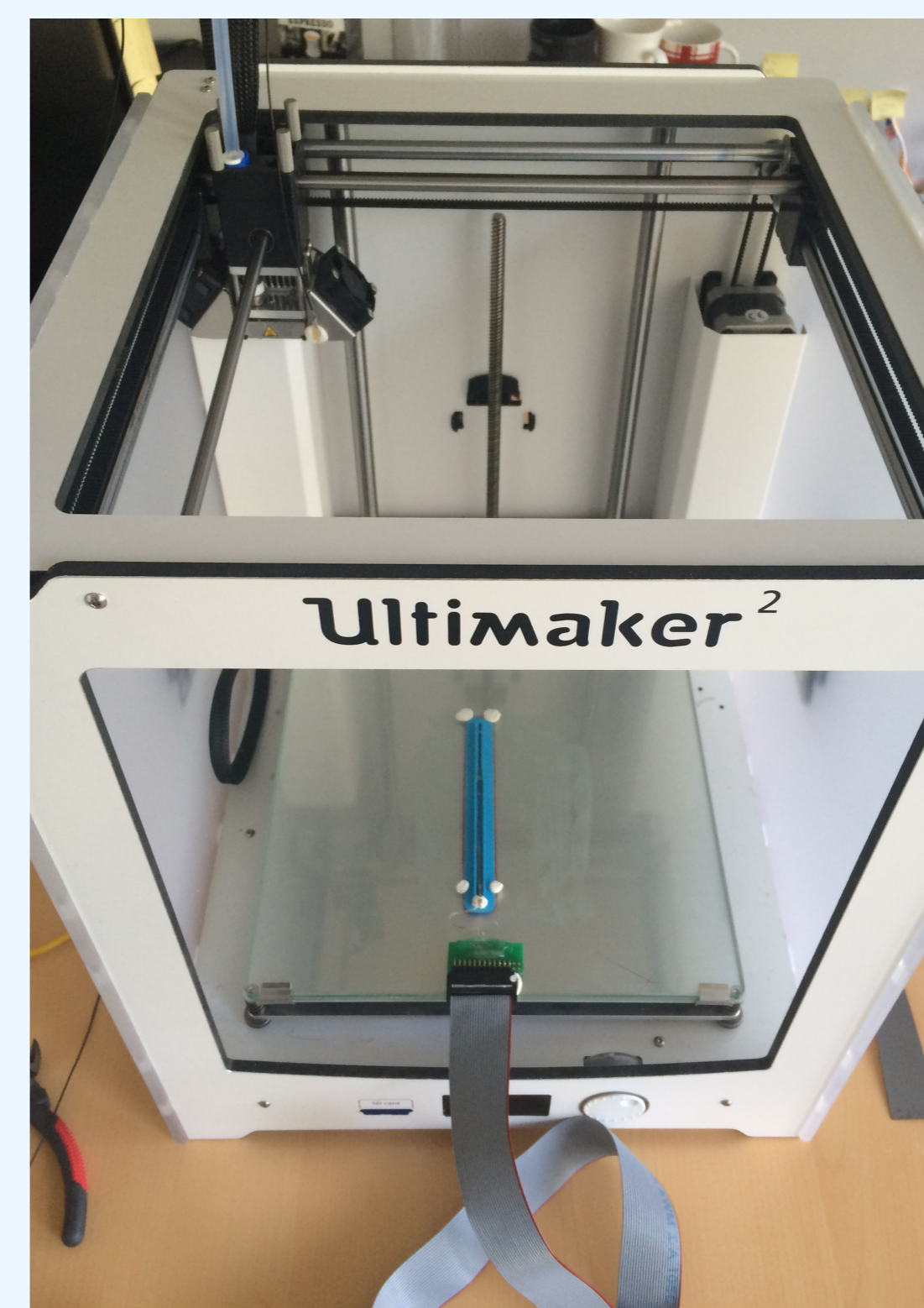
(b) 3-D printer for probe positioning
