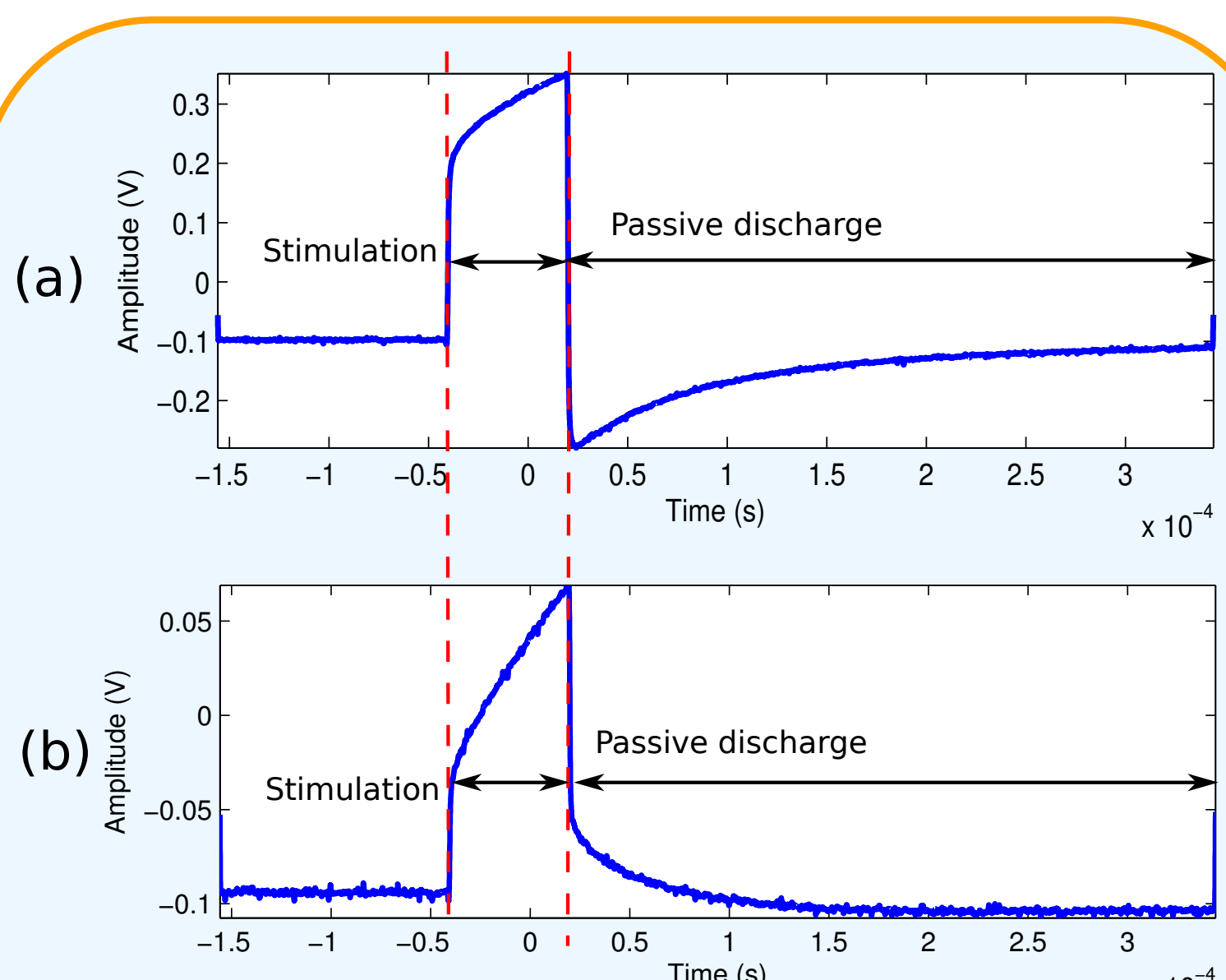
Figure 4. Stimulation waveform measured from: (a) near a stimulating electrode; (b) near a non-stimulating electrode
