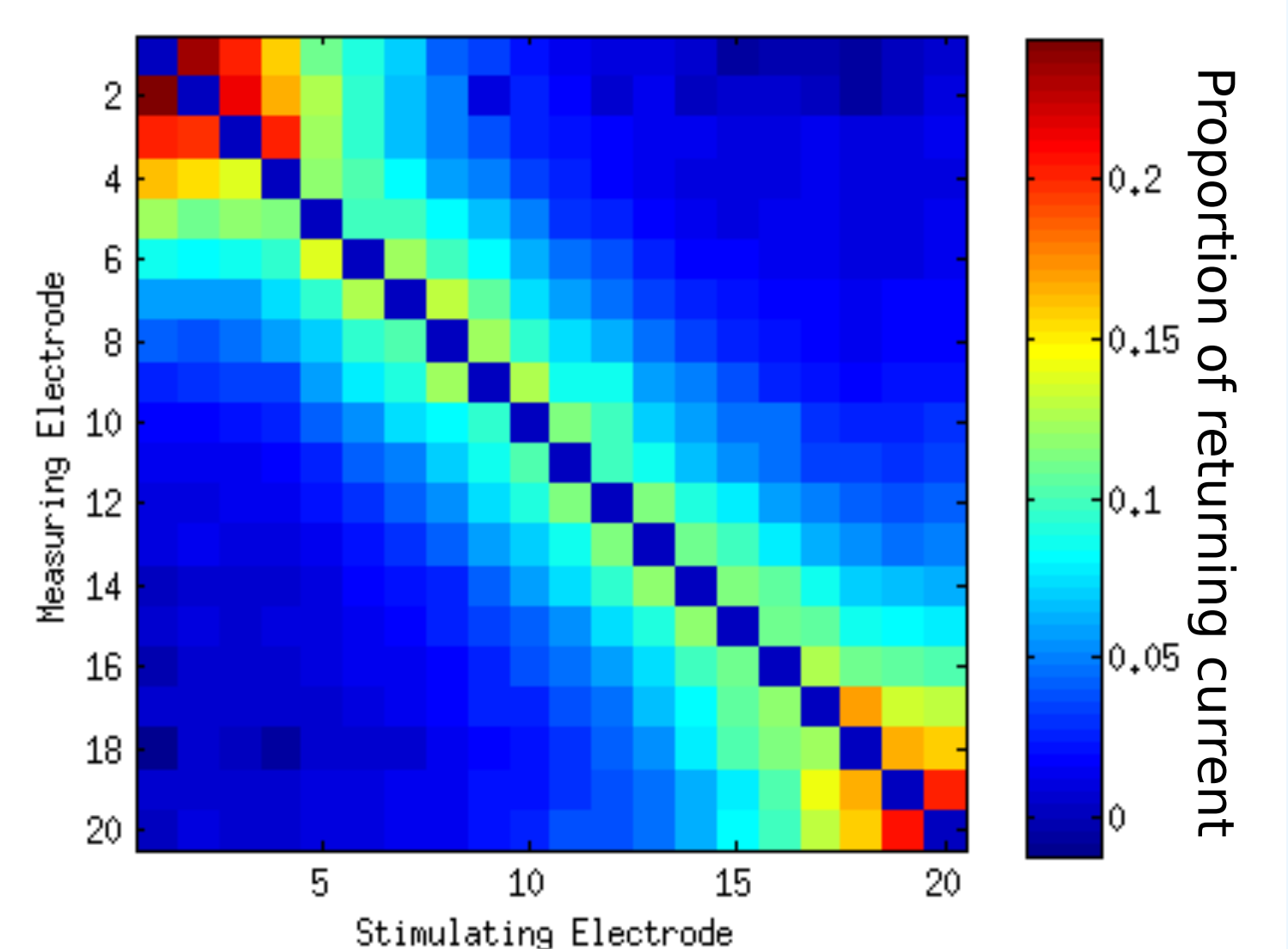
Figure 6. Returning current distribution from in situ measurements
