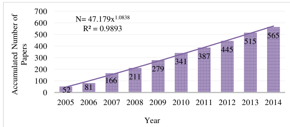
Fig. 1. Accumulated number of papers over a 10 Year Period. N being the accumulated number of papers and x stands for ordinal number of conferences.
